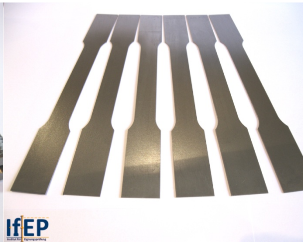
Flat test specimens
